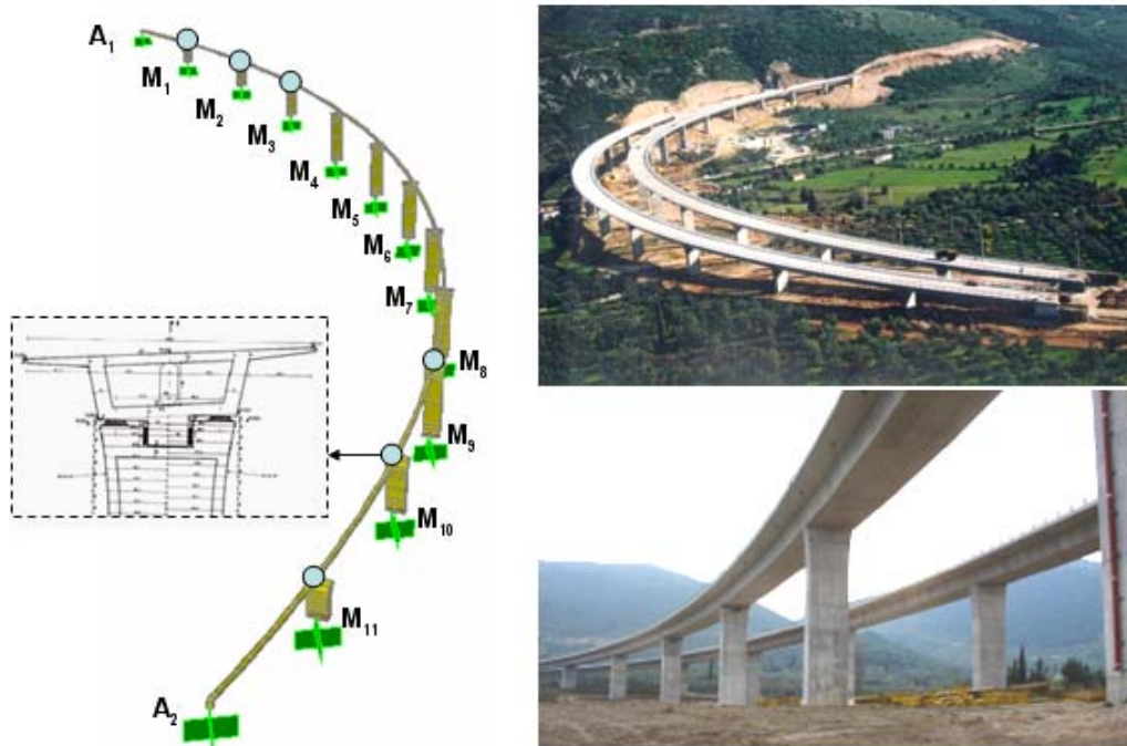
Figure 2: Layout of the bridge configuration and finite element modelling
