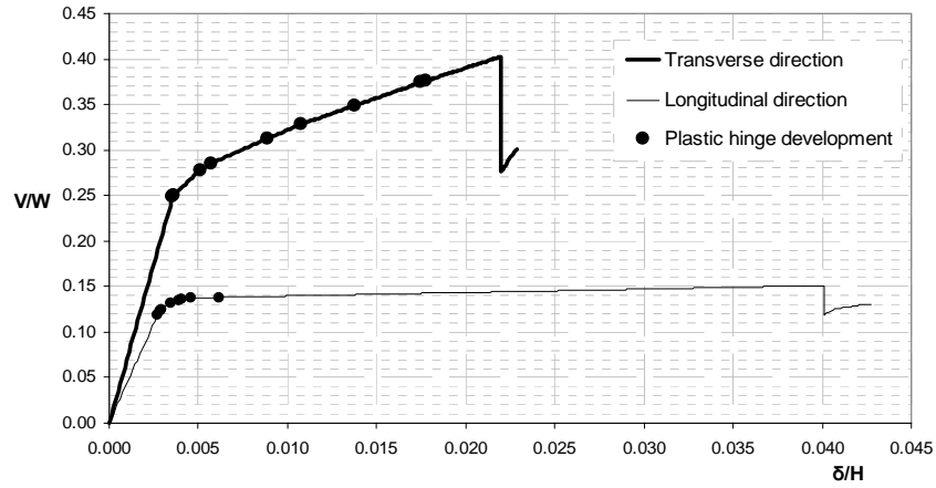
Figure 3: Base shear vs. pier top displacement, and sequence of plastic hinge formation in both directions of the bridge.
