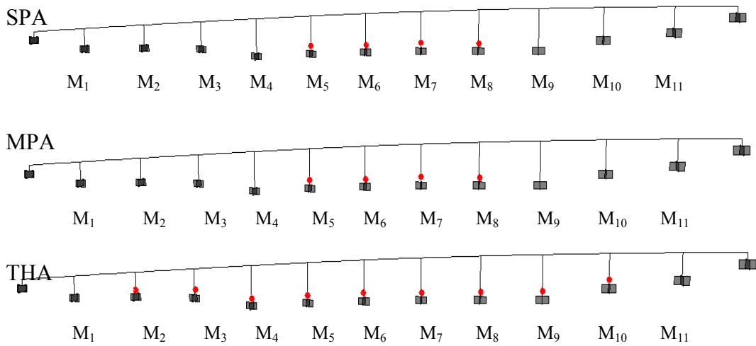
Figure 11: Location of plastic hinges determined by (a) 'standard' pushover analysis (b) MPA considering four 'modes' and (c) by non-linear time history analysis
