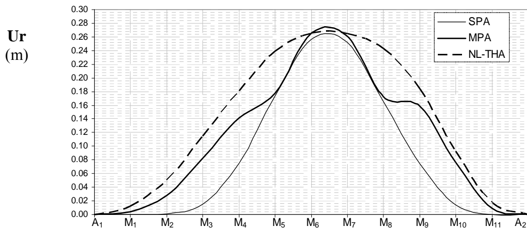
Figure 12: Pier top displacements by SPA, MPA and NL-THA. (transverse direction only), for 1.5 times the design earthquake intensity.
