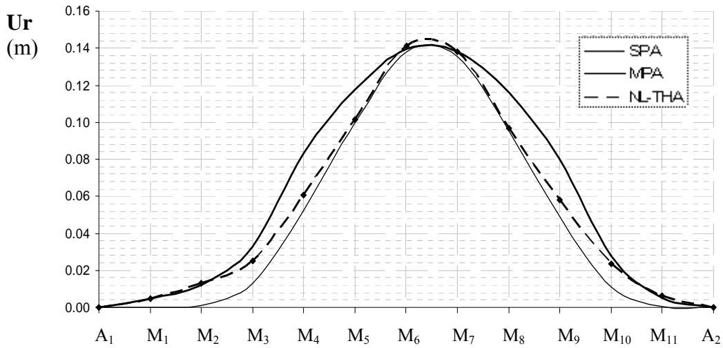
Figure 9: Pier top displacements calculated from SPA, MPA and THA, for elastic behaviour
