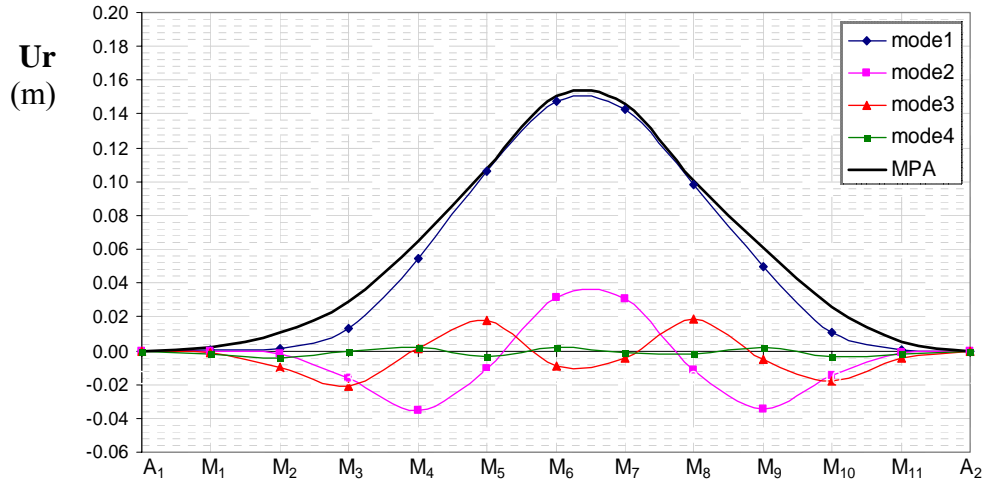
Figure 6: Pier top displacements according to MPA procedure for the design earthquake intensity (excitation in transverse direction only)
