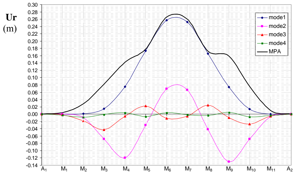
Figure 8: Pier top displacements according to MPA procedure for twice the design earthquake intensity. (transverse direction only)
