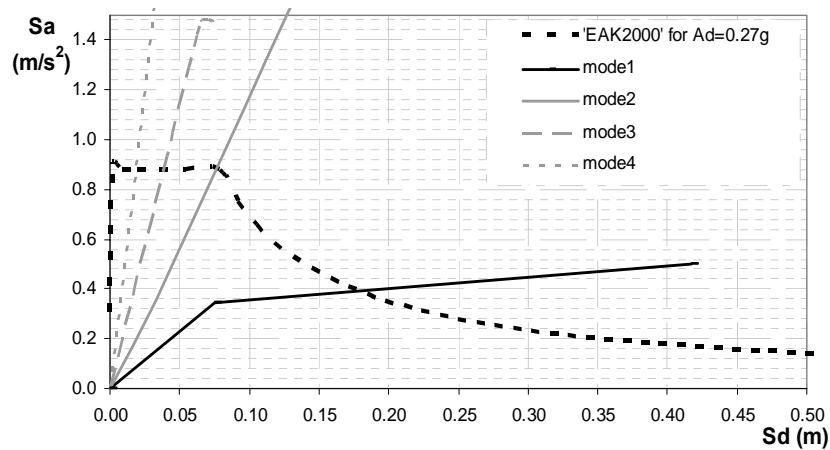
Figure 5: Capacity curves derived with respect to the central pier top for the four transverse modes (the elastic spectrum of the design earthquake is also shown)
