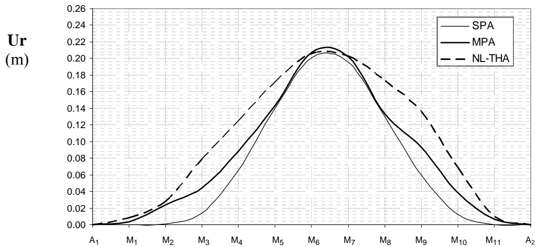
Figure 12: Pier top displacements by SPA, MPA and NL-THA. (transverse direction only), for 1.5 times the design earthquake intensity.
