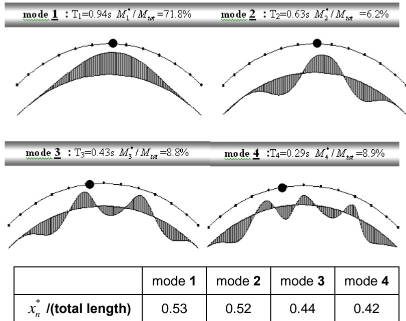
Figure 4: Force distribution, s_n^* = \mathbf{m}\phi_n , location of the equivalent SDOF systems and modal parameters for the main transverse modes of the bridge
