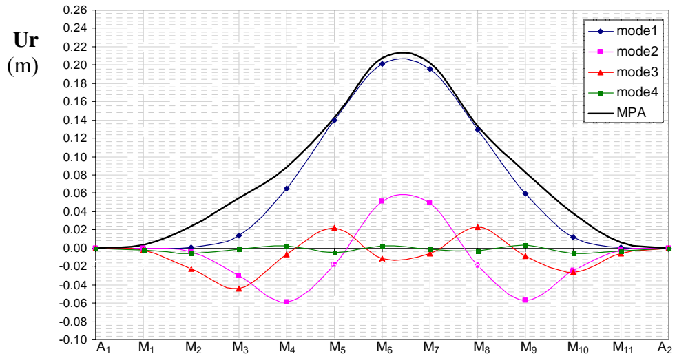
Figure 7: Pier top displacements according to MPA procedure for 1.5 times the design earthquake intensity (transverse direction only)
