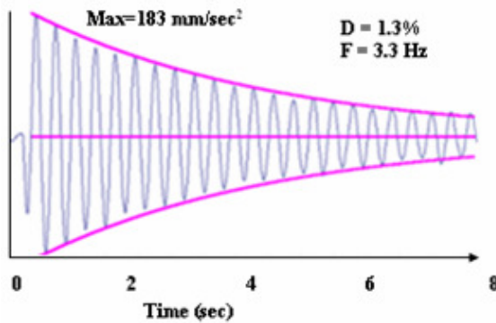
Figure 5a. Low intensity pull-out test. (structure with cables and no extra mass).
