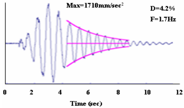
Figure 5b. Low-to-medium intensity forced vibration test that produced the pier damage (structure with cables and extra mass).
