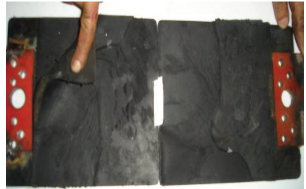
Figure 13. The unbonding of the elastomer from the steel plating at the end of this loading sequence.
