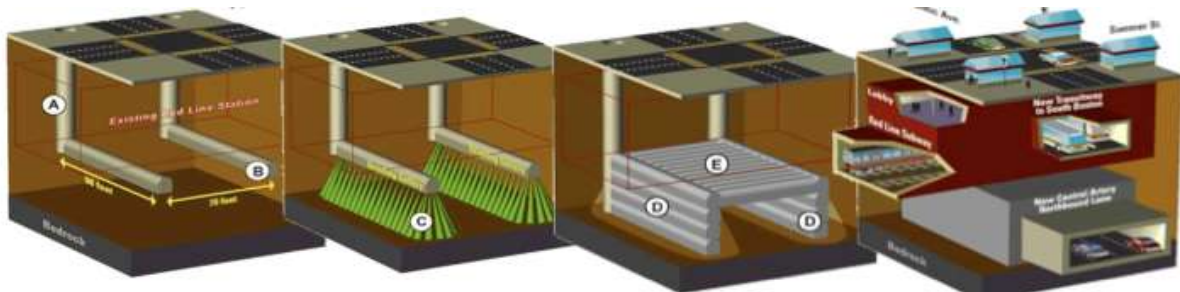
Figure 4. Example of station underpinning according to the novel solution of the Central Artery/Tunnel Project (CA/T) of the Boston Subway.
