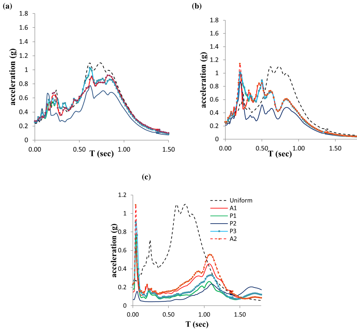
Figure 3: Acceleration response spectra of Northridge No2 ground motion recorded at the free surface of (a) Type B, (b) Type C and (c) Type D geological profile vs Uniform excitation (Type A).
