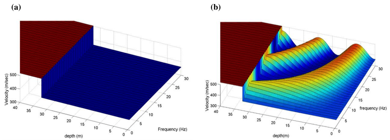
Figure 4: Velocity distribution of the subsoil structure: (a) Type C and (b) Type D geological profile.
