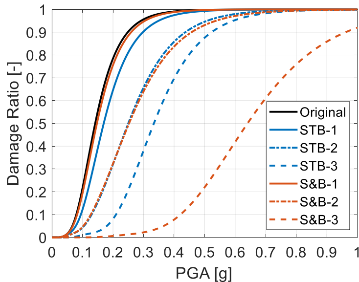
Figure 3 - Vulnerability curves for different retrofitting solutions and incremental phases
