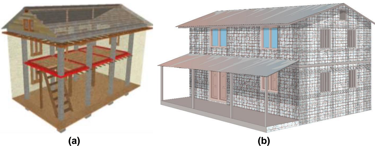
Figure 1 - Retrofitting strategies in Nepal: (a) Strongback (STB), (b) Splint and Bandage (S&B)
